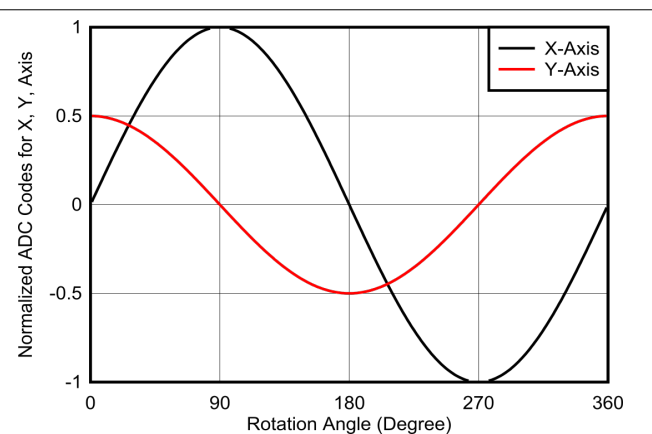
Figure 8-18. X and Y Sensor Data for Full 360 Degree Rotation for Off-Axis Measurement
