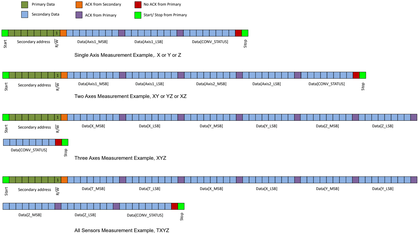
Figure 7-11. 1-Byte I 2 C Read Command for 16-Bit Data With CRC Disabled, CRC_EN = 0b
