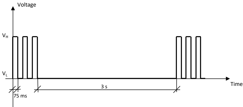
Figure 5: GPIO pin progress for registered home network 4G
