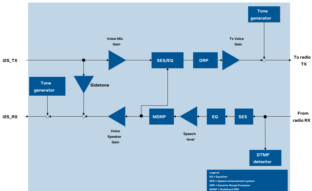
Figure 13: LARA-L6004 / LARA-R6001 / LARA-R6401 / LARA-R6801 speech processing system
