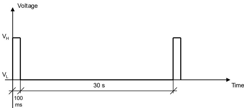
Figure 6: GPIO pin progress for registered home network NB-IoT
