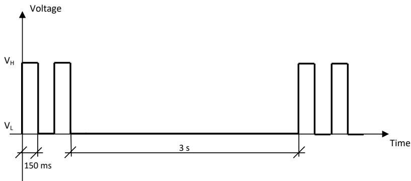
Figure 9: GPIO pin progress for registered roaming 4G
