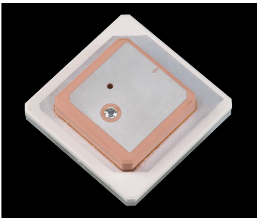
Figure 68: Ceramic stack
