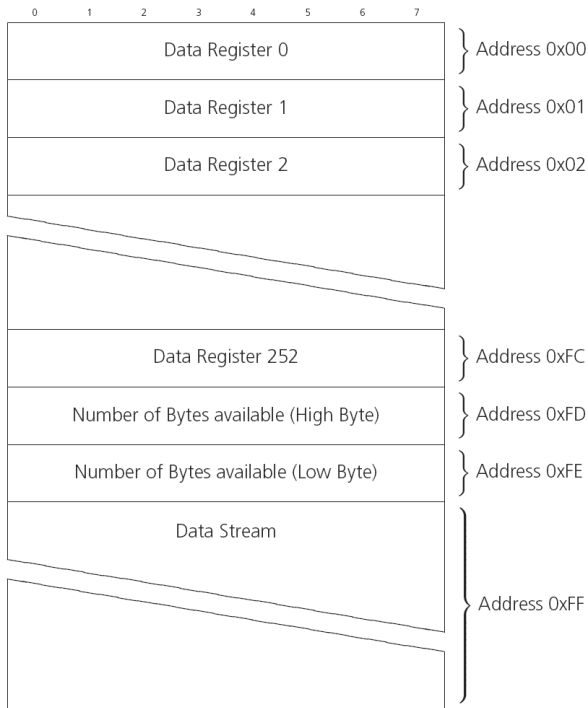
Figure 18: I2C register layout
