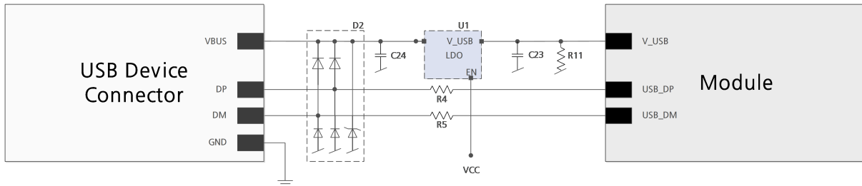
Figure 23: ZED-F9P example circuit for USB interface
