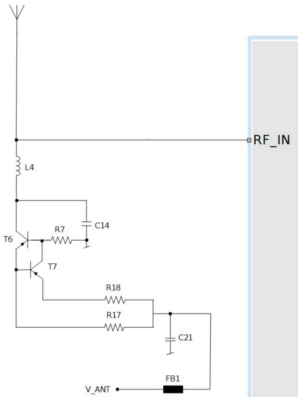
Figure 44: ZED-F9P with external voltage antenna bias and current limit circuit
