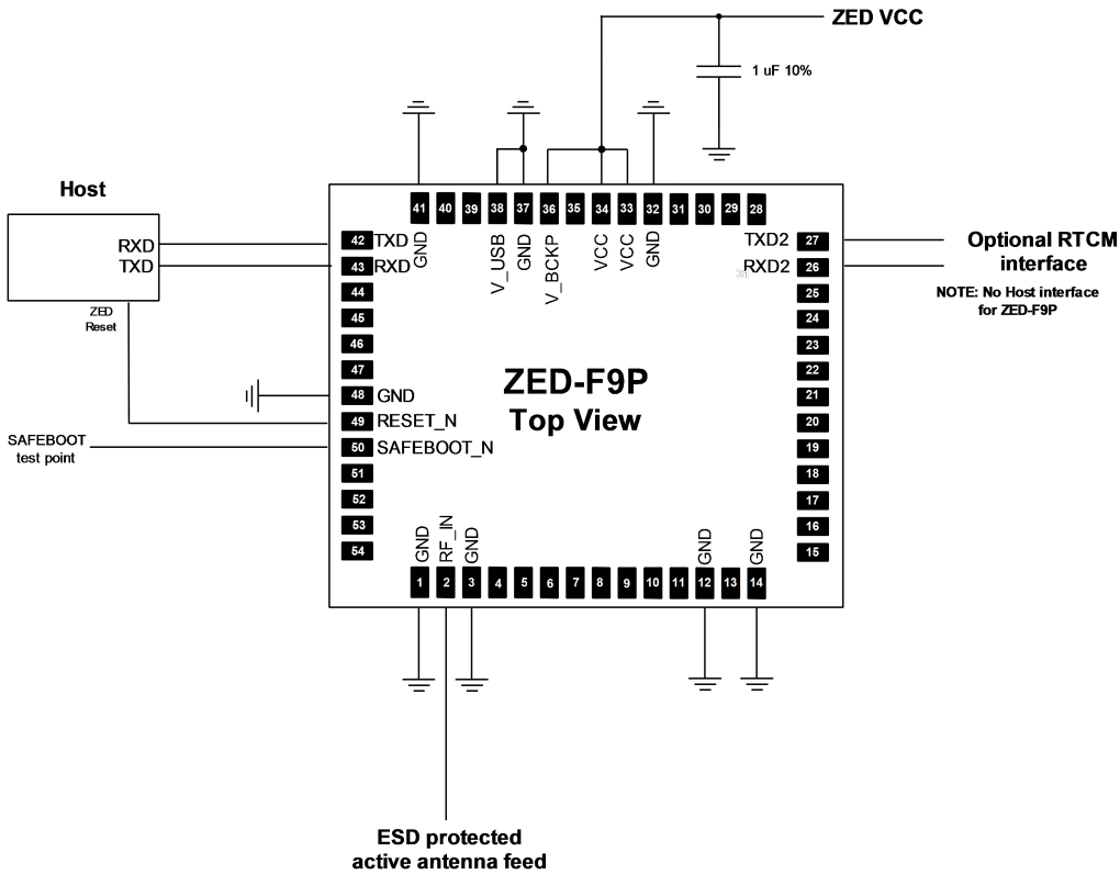
Figure 40: Minimal ZED-F9P design
