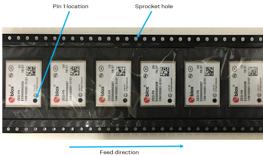
Figure 55: Orientation of ZED-F9P on the tape
