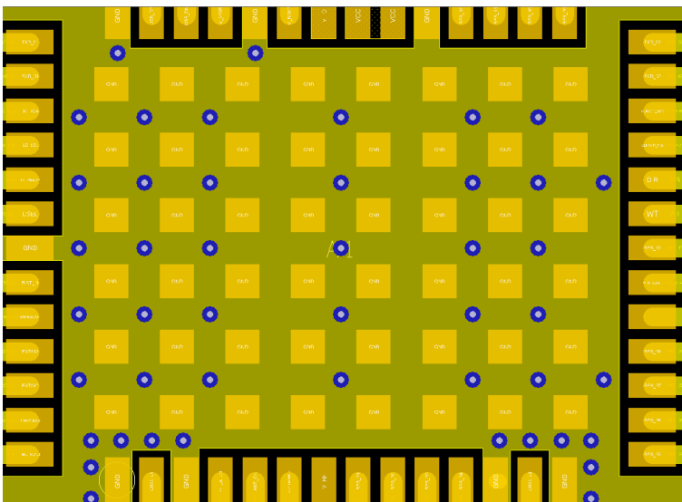
Figure 52: Top layer fill and vias
