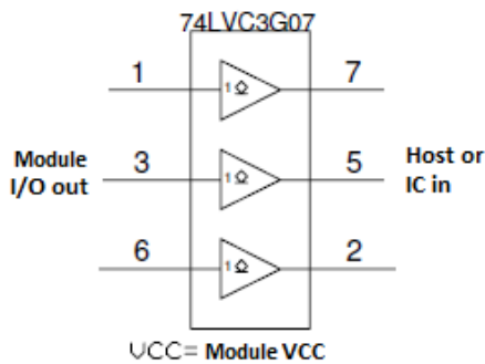
Figure 16: ZED-F9P output isolation
