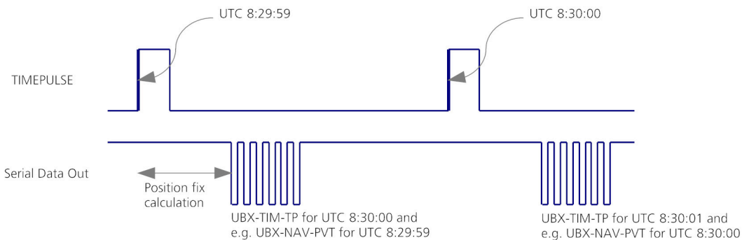
Figure 25: Time pulse and TIM-TP
