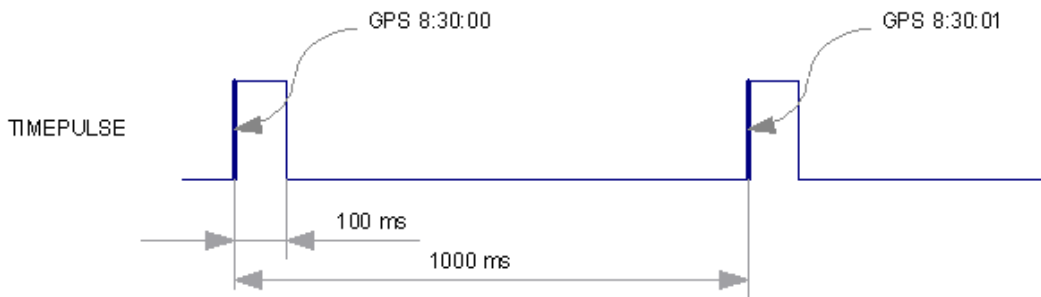
Figure 26: Time pulse signal with the example parameters
