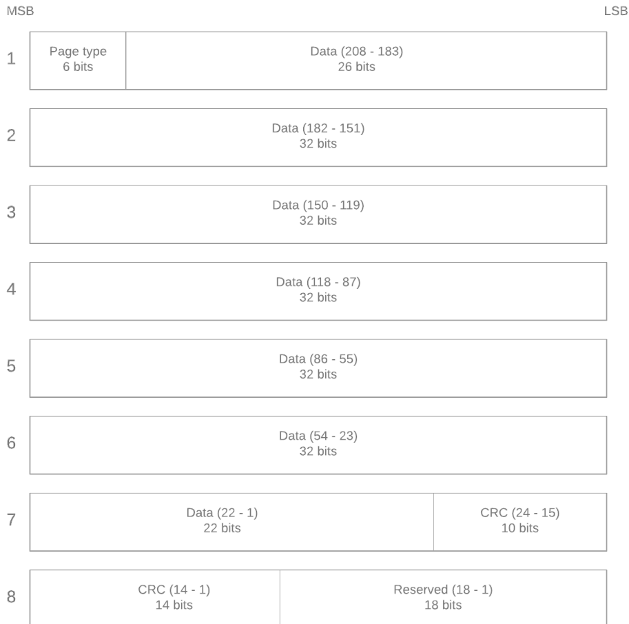
Figure 35: Galileo E5a subframe words
