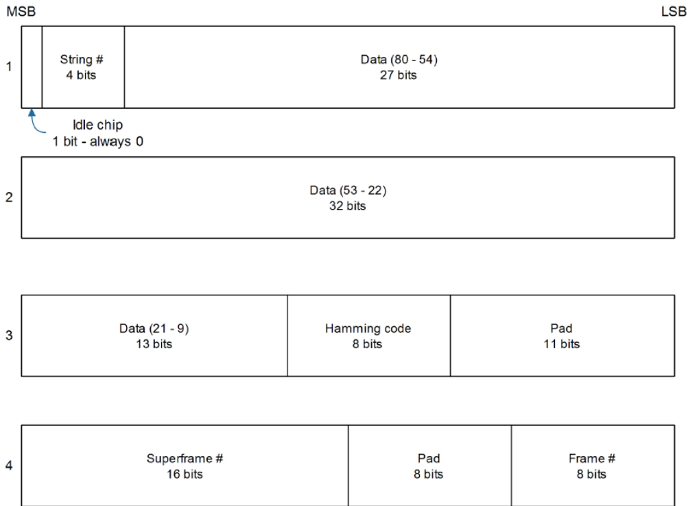
Figure 31: GLONASS navigation message data
