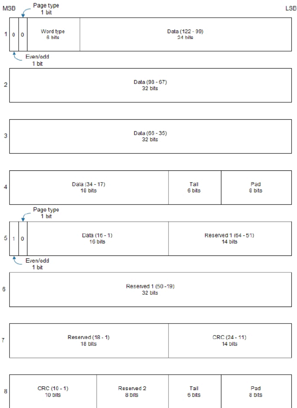
Figure 34: Galileo E5b subframe words
