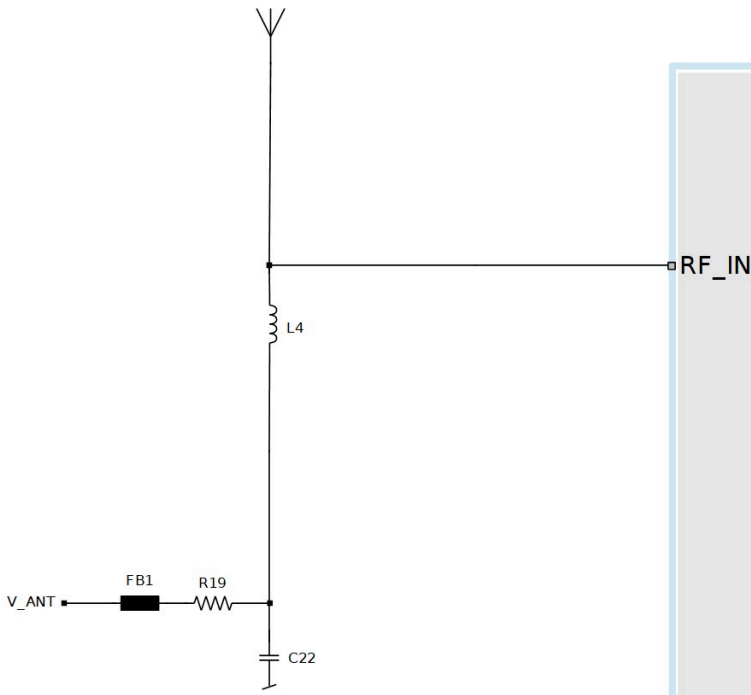
Figure 43: ZED-F9P with external voltage antenna bias
