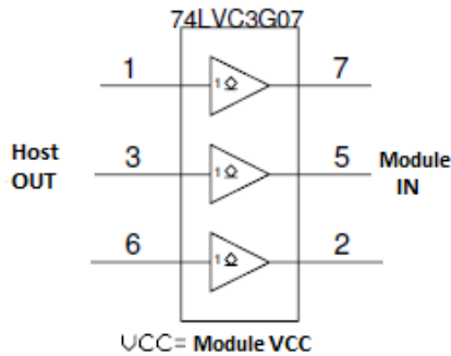
Figure 17: ZED-F9P input isolation
