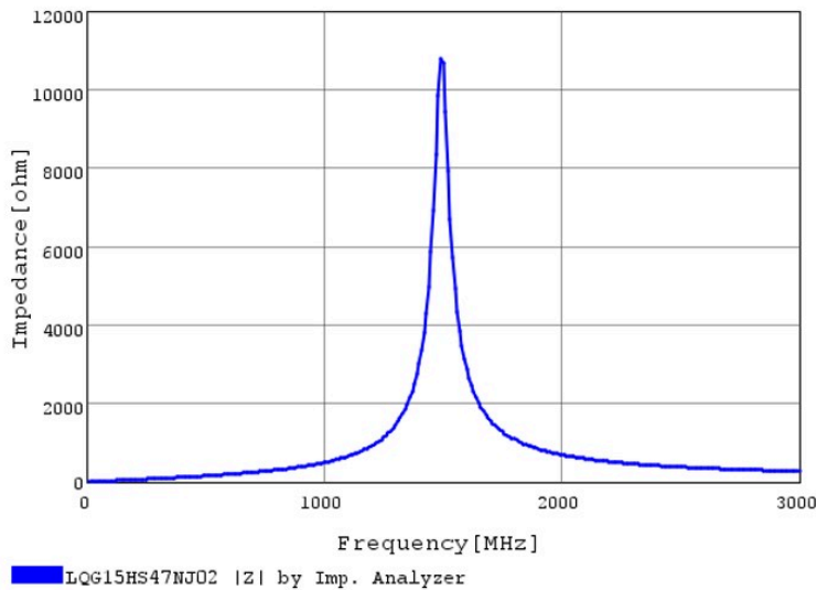
Figure 42: ZED-F9P antenna bias inductor impedance
