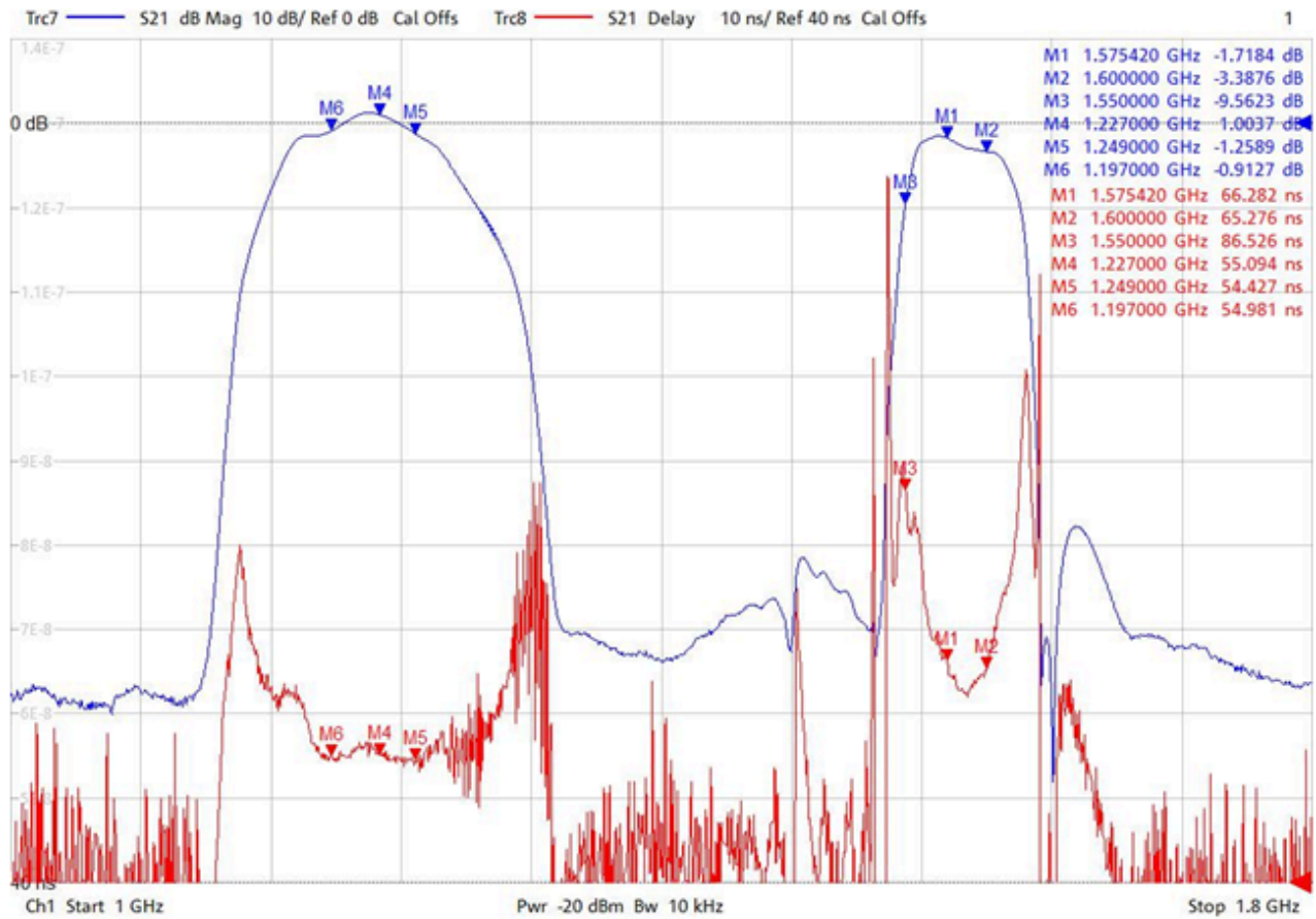
Figure 69: Low-cost L1/L2 antenna band characteristics
