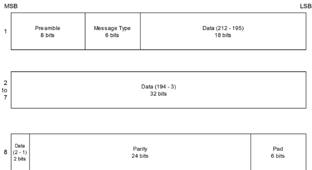
Figure 36: SBAS subframe words
