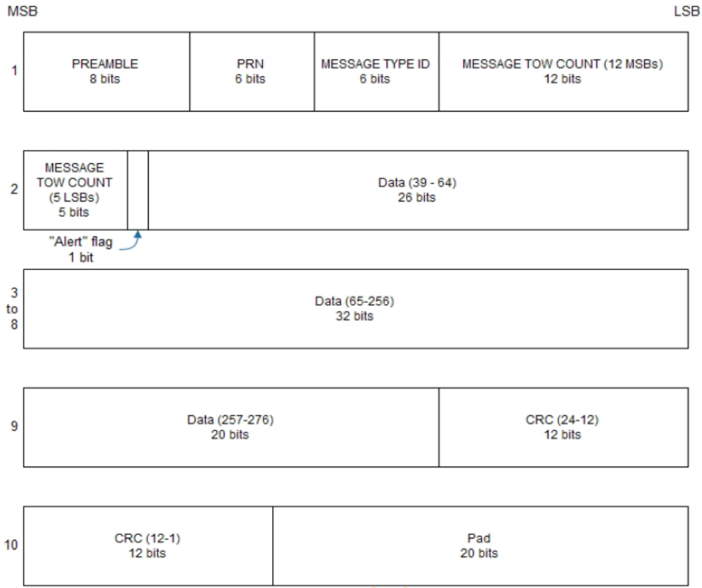
Figure 30: GPS L5 subframe words
