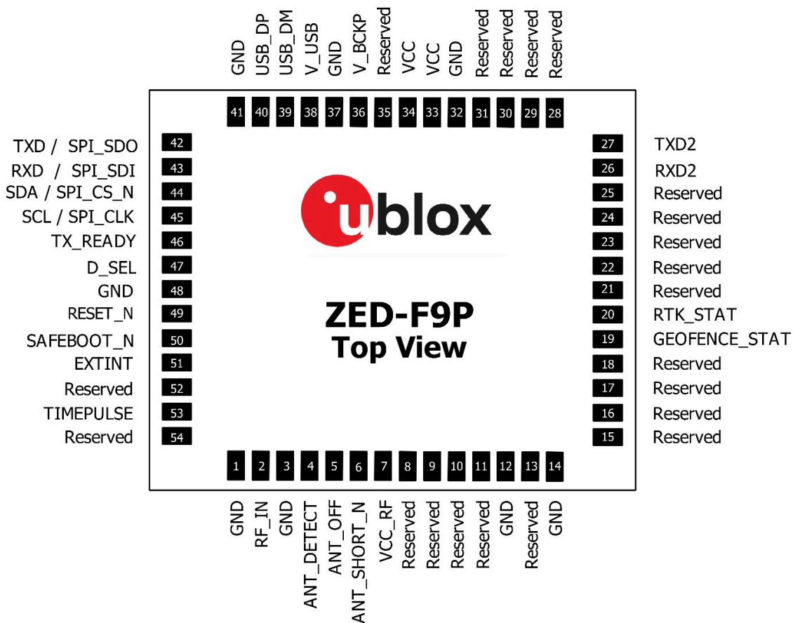
Figure 38: ZED-F9P pin assignment
