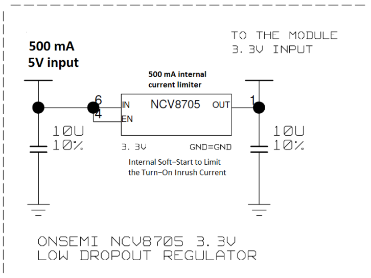
Figure 39: ZED-F9P power supply
