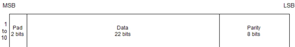
Figure 32: BeiDou subframe word
