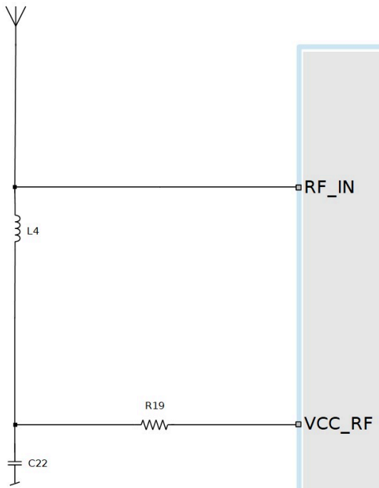
Figure 45: ZED-F9P VCC_RF antenna bias
