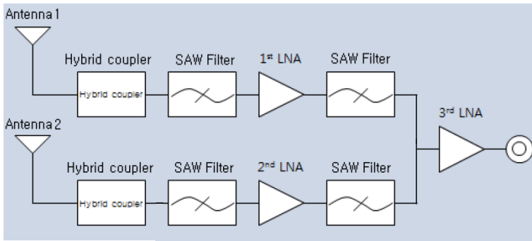
Figure 41: u-blox low cost dual-band antenna internal structure
