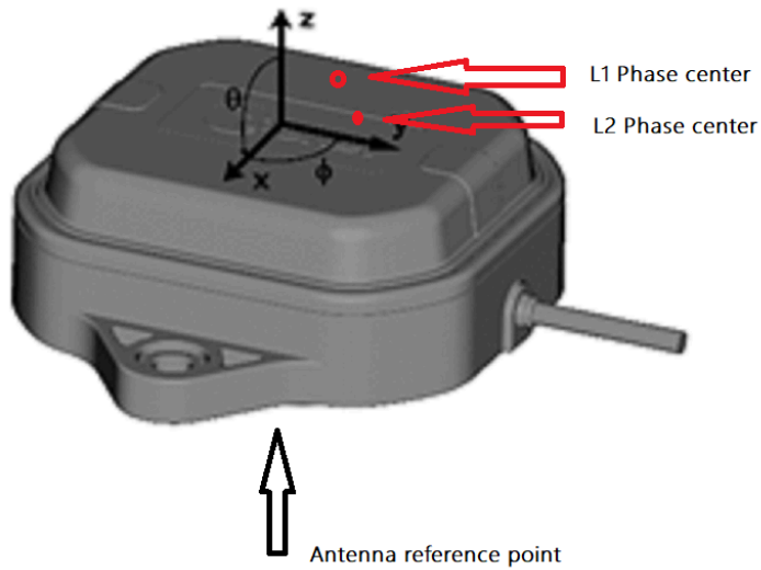
Figure 67: Stacked patch antenna
