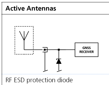
Figure 47: RF ESD precautions
