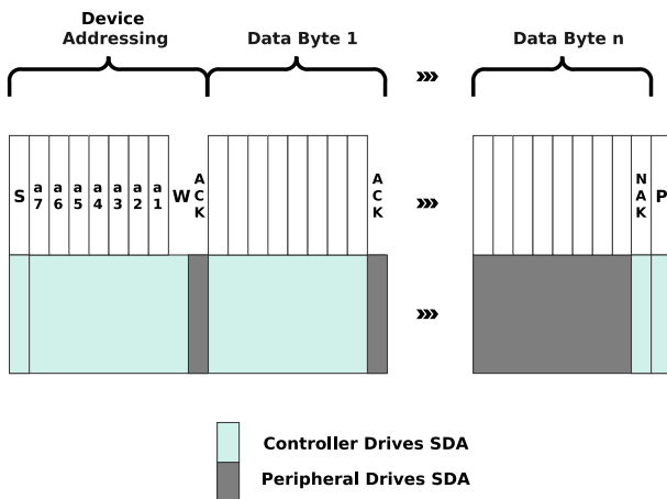
Figure 21: I2C write access
