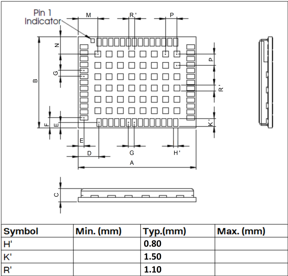
Figure 49: ZED-F9P suggested footprint (i.e. copper mask)
