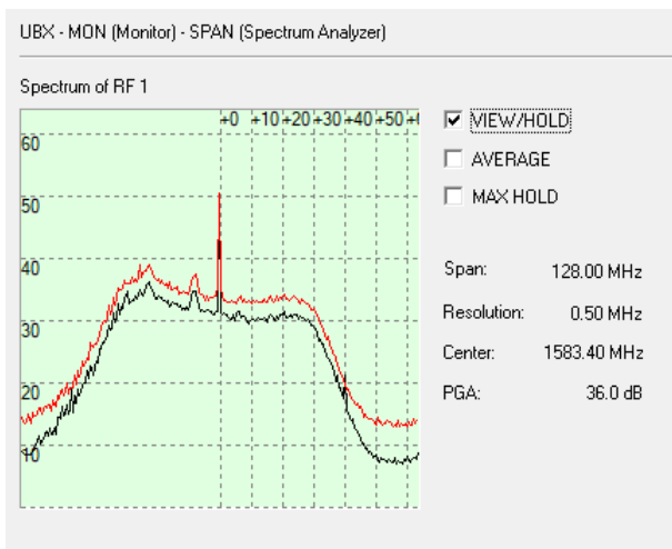
Figure 37: Spectrum analyzer view in u-center with the option view/hold selected
