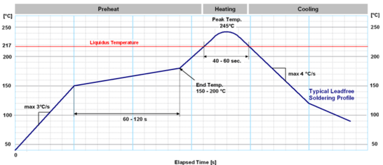
Figure 54: Soldering profile for professional grade ZED-F9P
