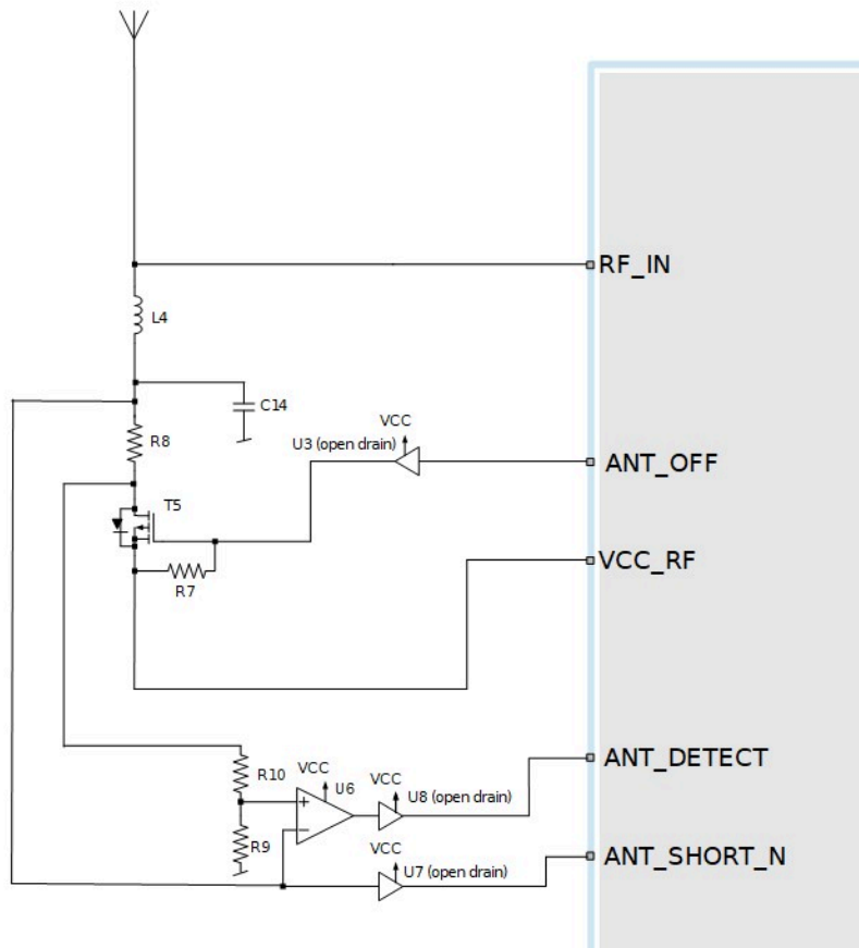
Figure 46: ZED-F9P antenna supervisor circuit
