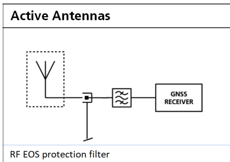
Figure 48: Active antenna EOS protection
