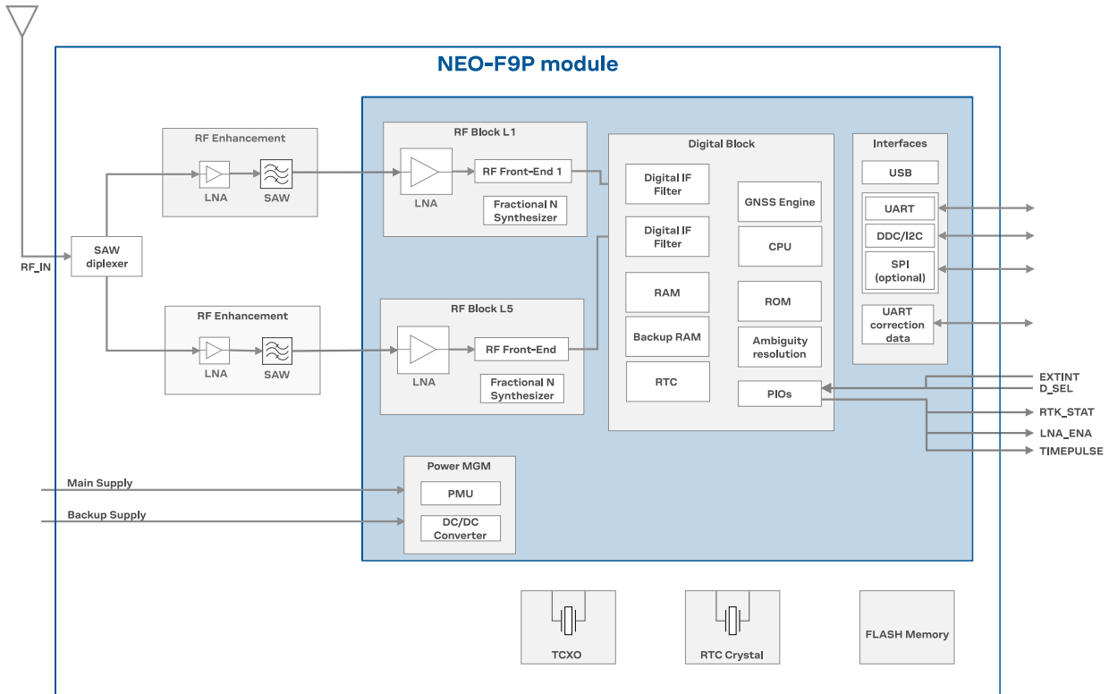
Figure 1: NEO-F9P-15B block diagram
